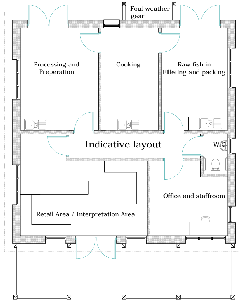
FLOOR PLAN
