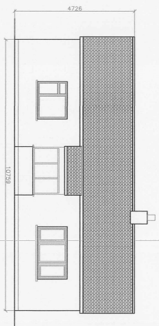
West Elevation
