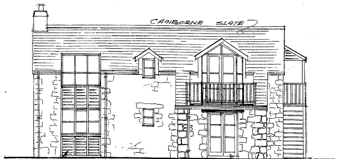
FRONT ELEVATION
