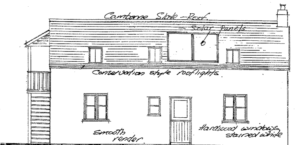
REAR ELEVATION
