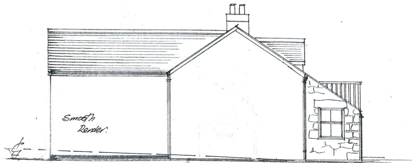
NORTH ELEVATION
