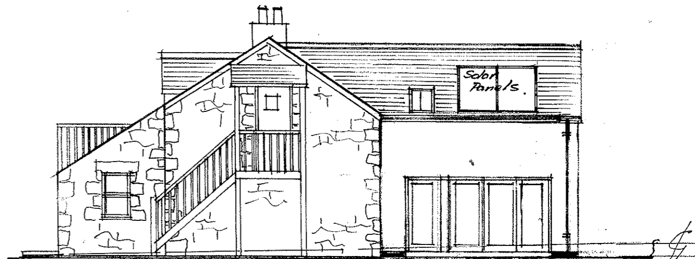
SOUTH ELEVATION
