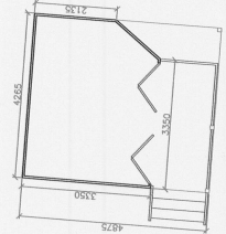
Garden Shed Plan
