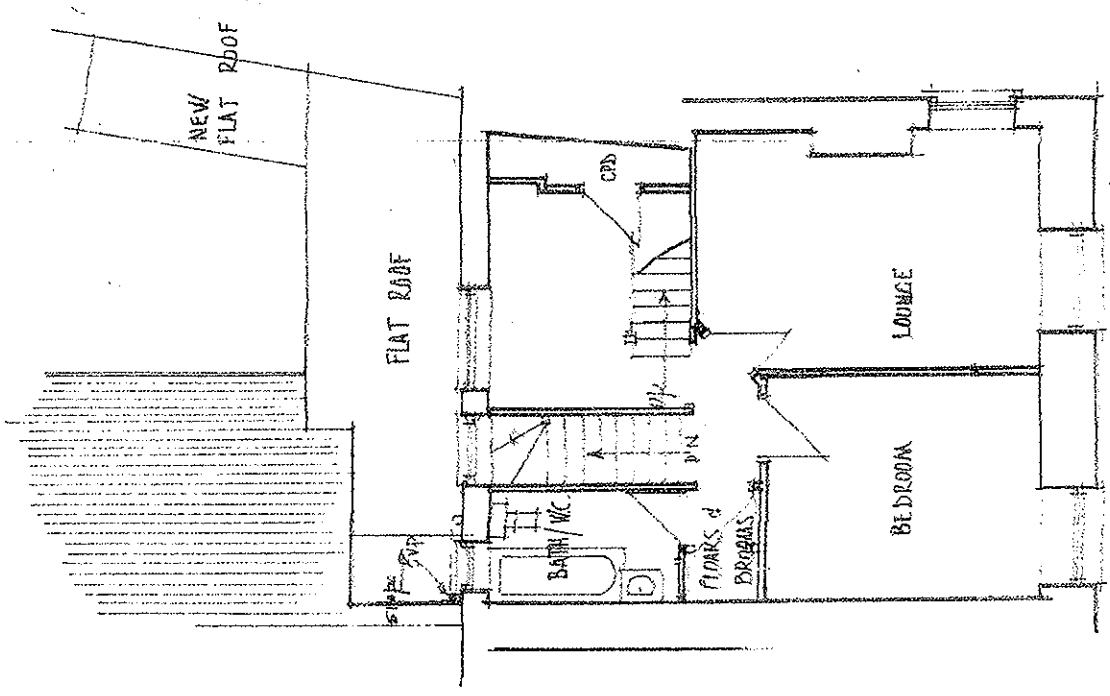
EXISTING & PROPOSED FIRST FLOOR LAYOUT
