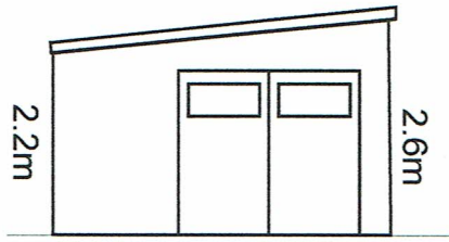
East Elevation
