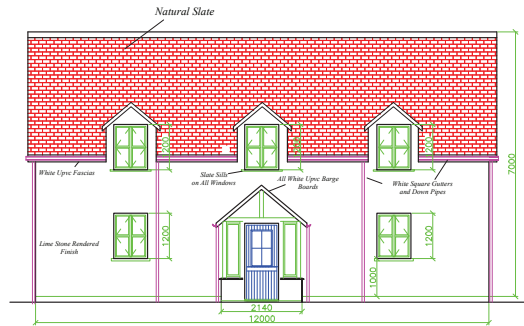
South Elevation
