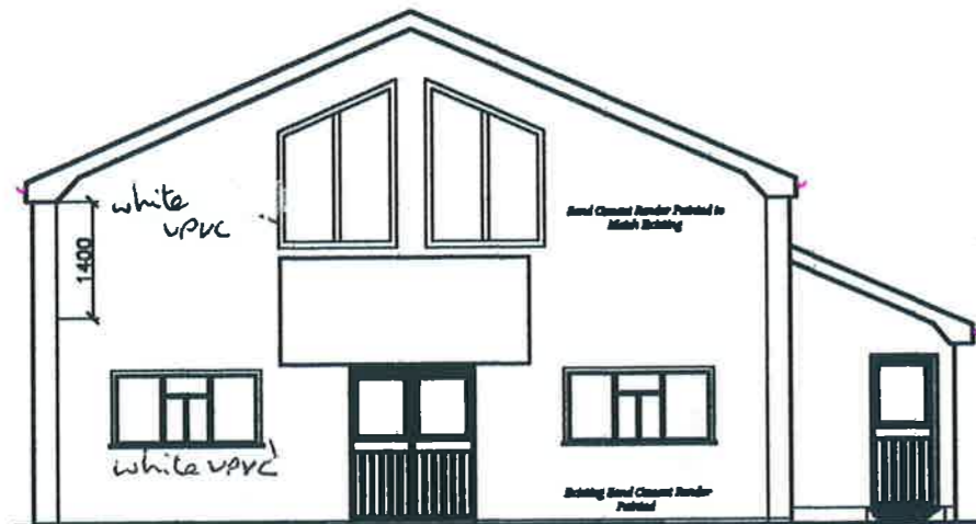
NORTH ELEVATION
