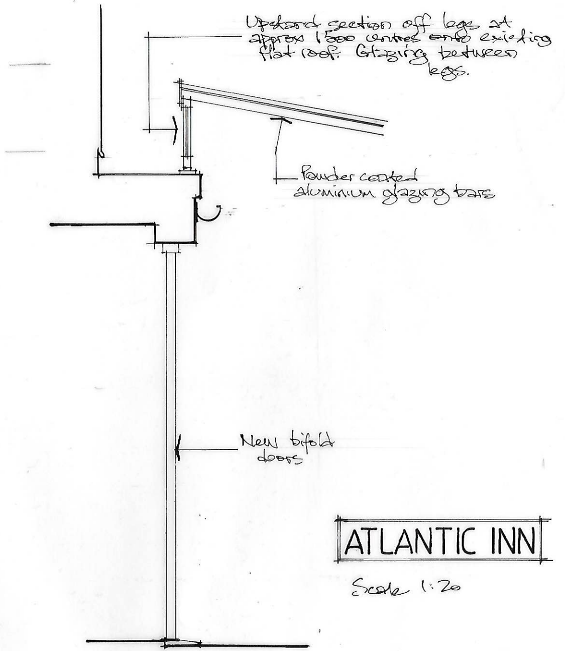
PROPOSED SECTION
