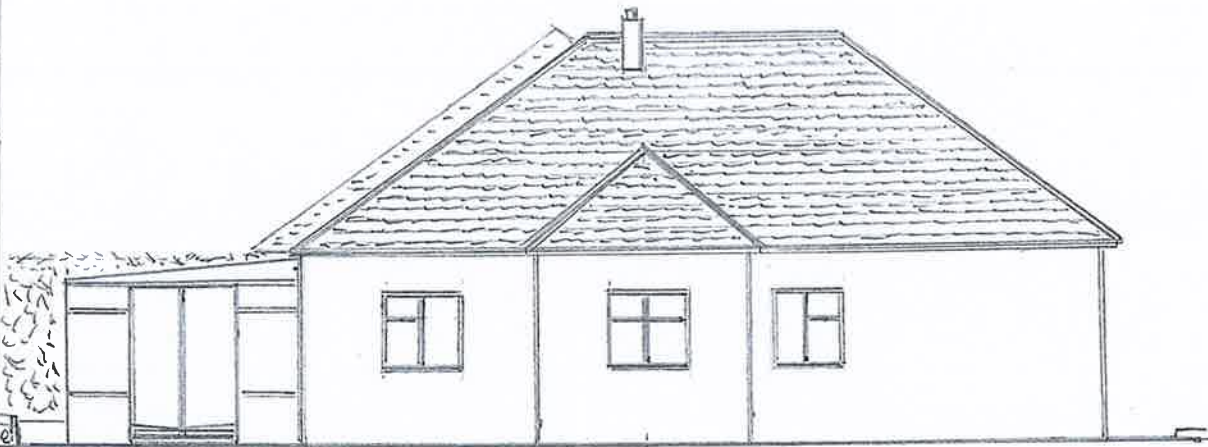
EAST ELEVATION
