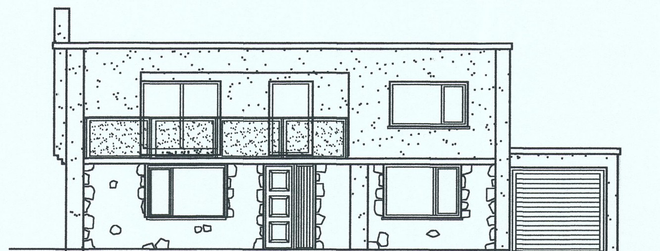
North Elevation
