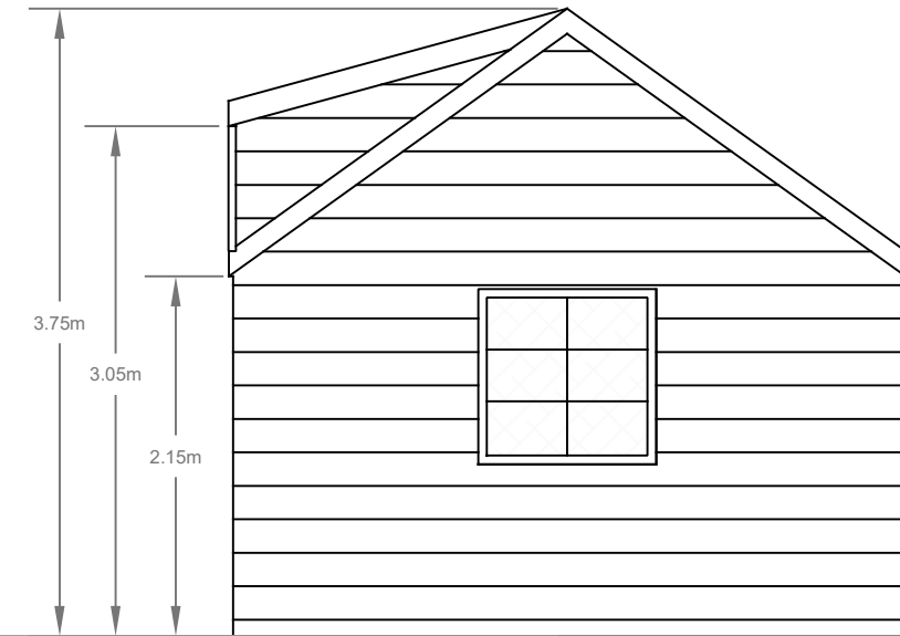
West Elevation
