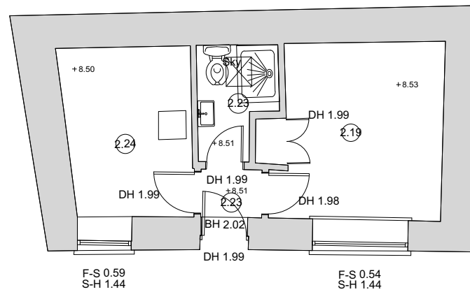
GROUND FLOOR (NORTH OUT BUILDING)
