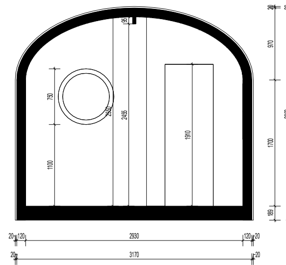
section A - 1:50
