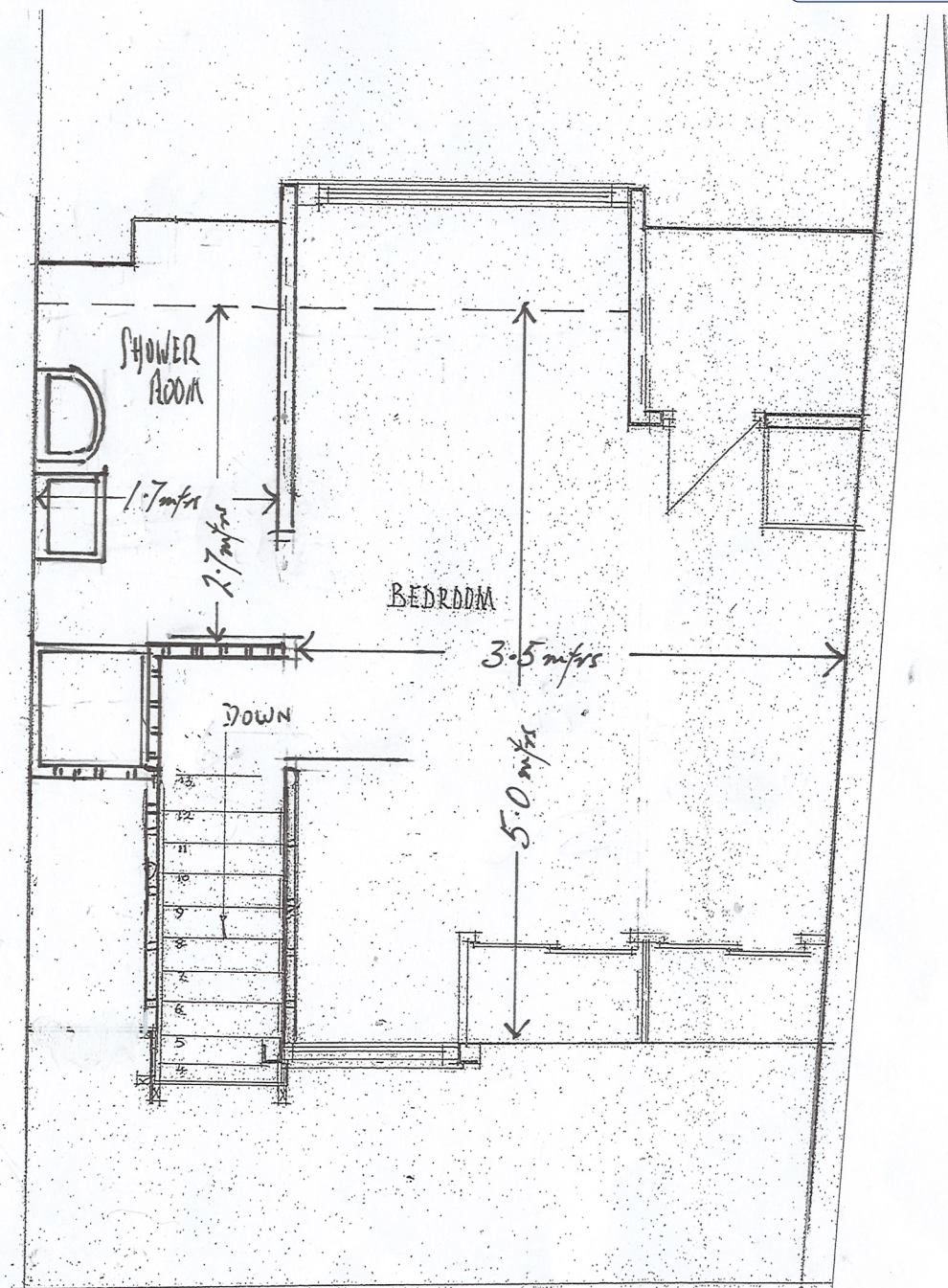
ST. MARVS SECOND FLOOR PLAN AS EXISTING SCALE 1/4" = 1'0"
