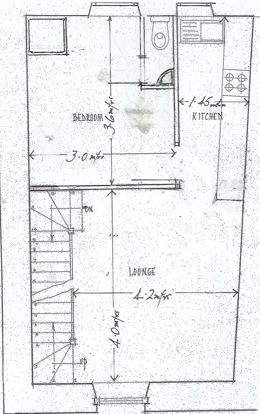
"SEA WAVES" 5, LOWER STRAND FIRST FLOOR PLAN AS EXISTING
