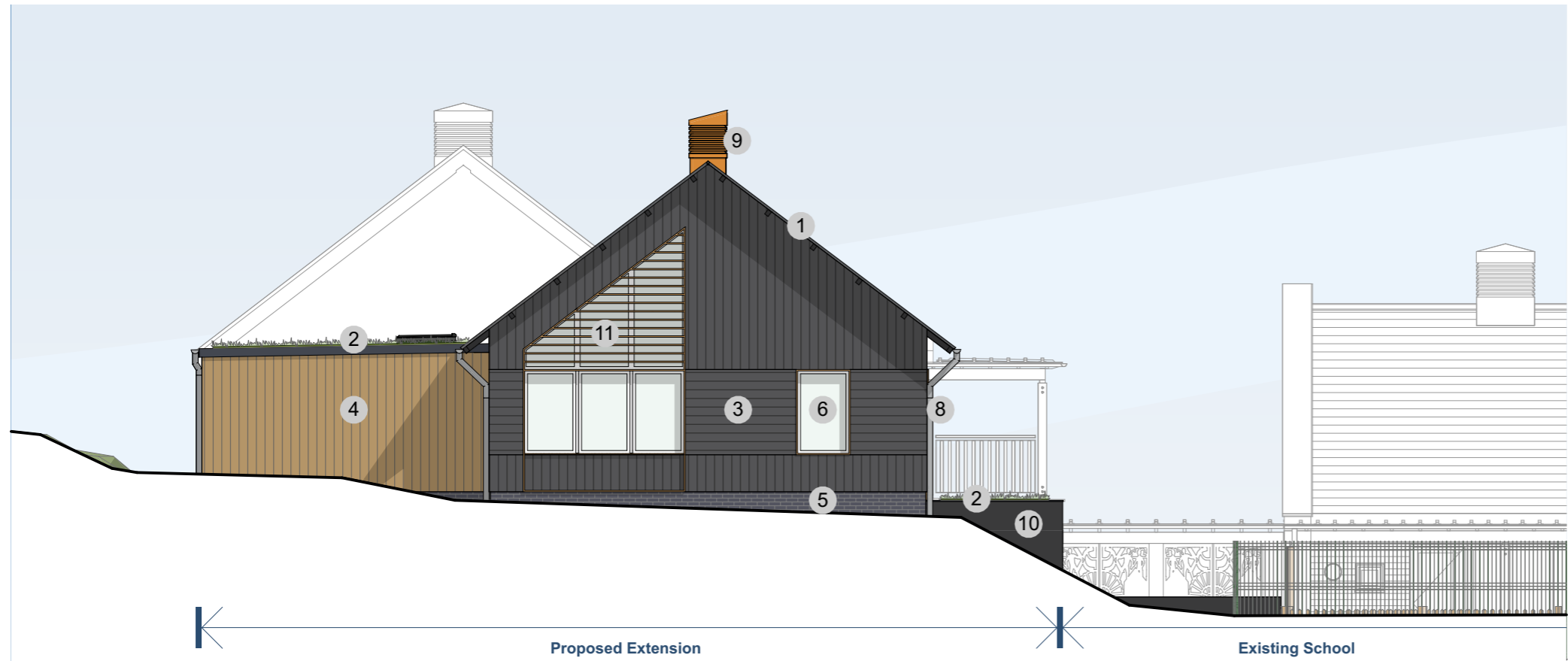
PROPOSED SOUTH ELEVATION
