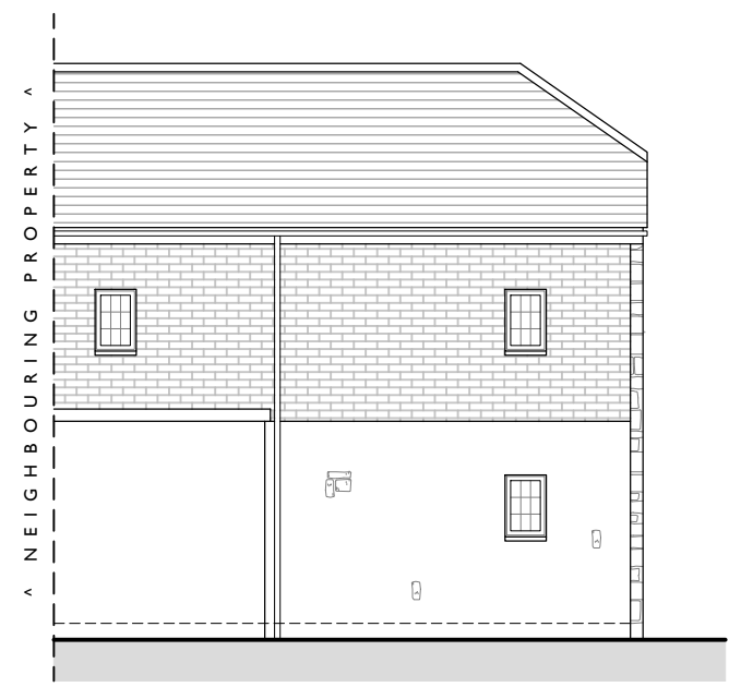
REAR ELEVATION - scale 1/100 (EXISTING)
