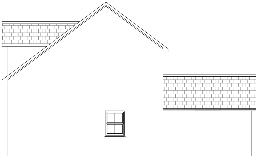
Right Elevation West-North
