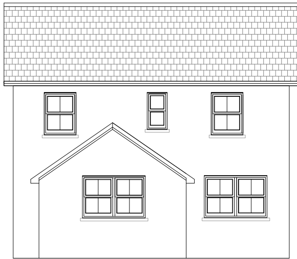
Front Elevation West-South
