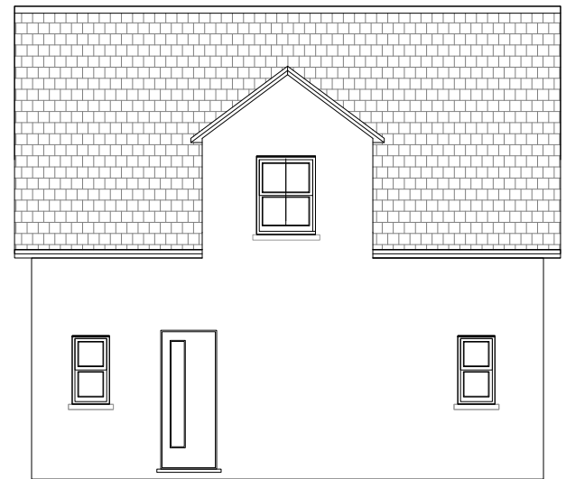
Rear Elevation North-East
