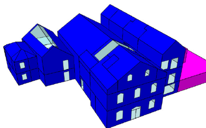
Figure 1: 3D view of the IES thermal model.
