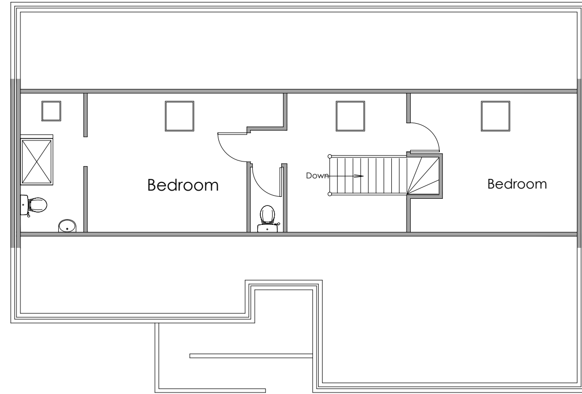
Second Floor area 51.84 SqM
