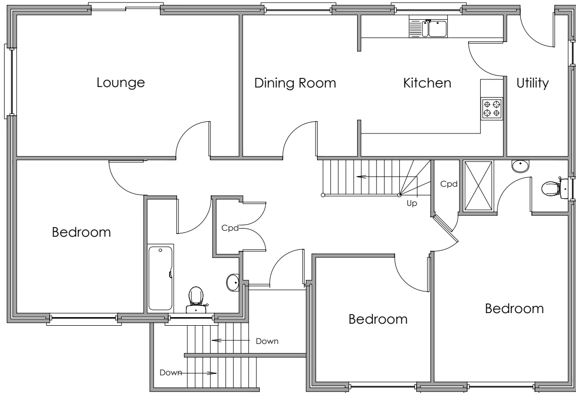
First Floor area 122.46 SqM
