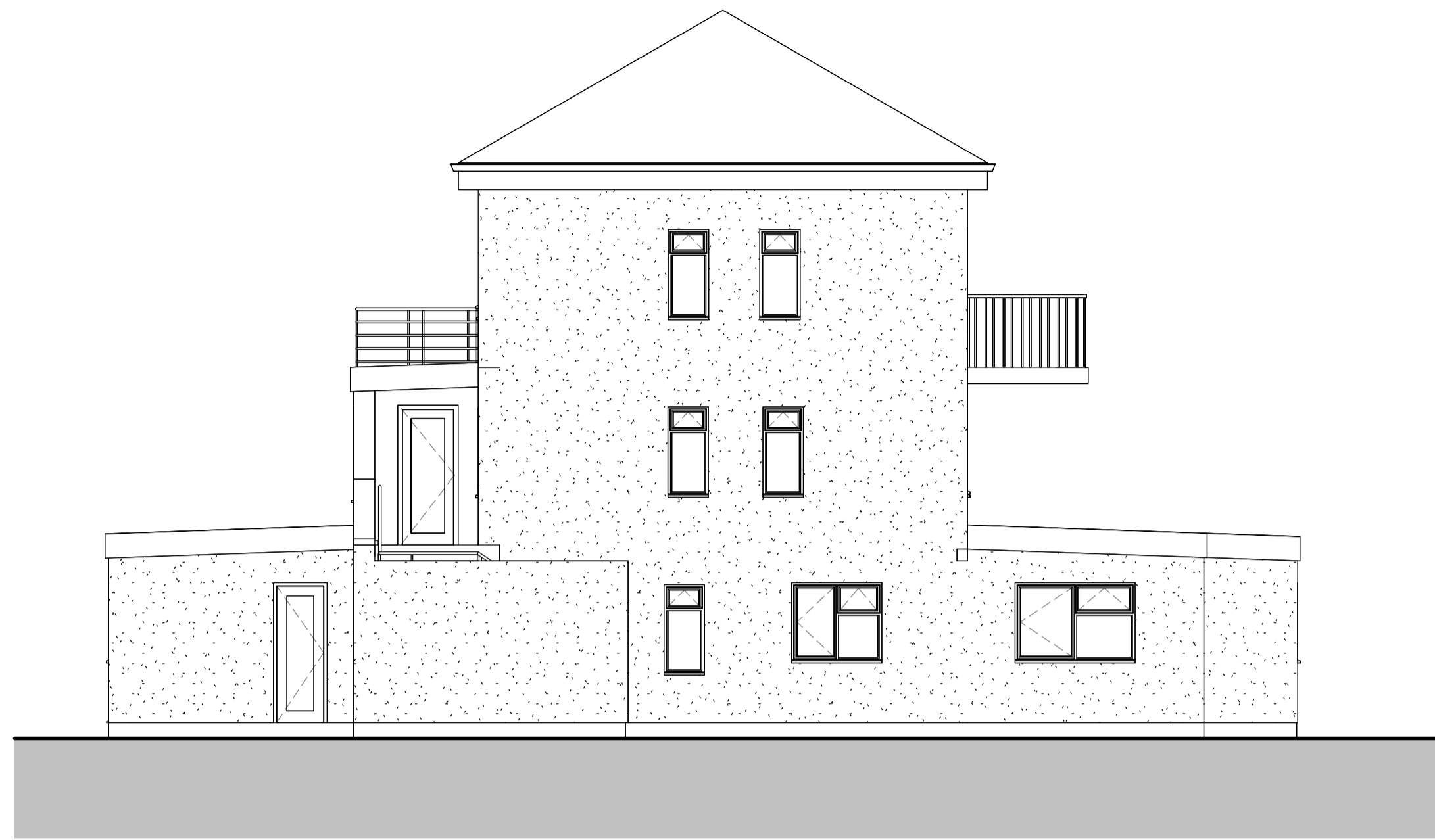
1 Existing East Elevation 1:75
