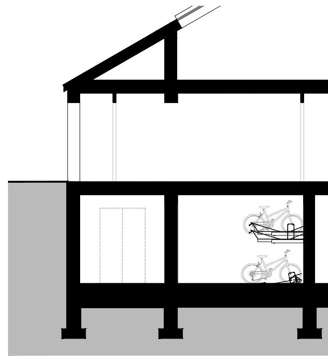
Indicative Section A
