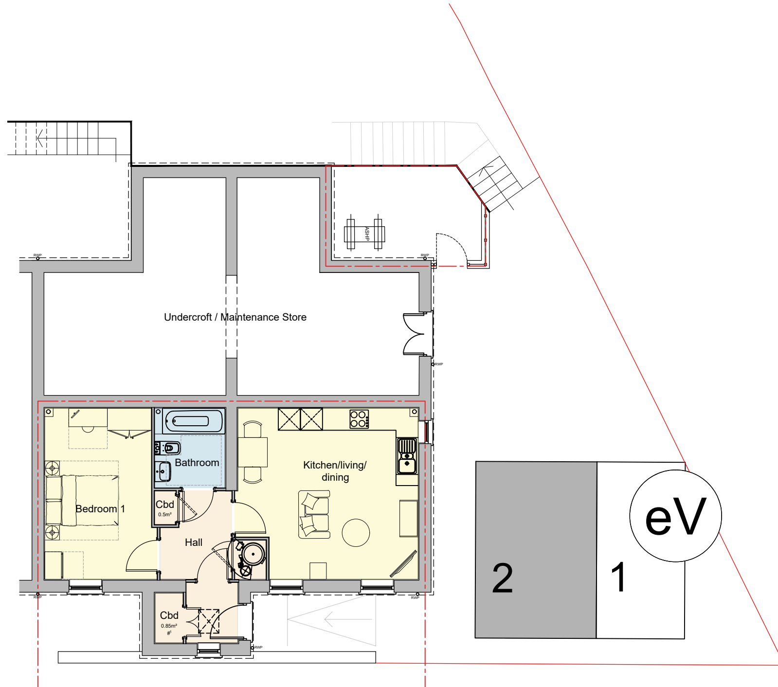
Type A - V2 Lower Ground Floor Plan M4(2)
