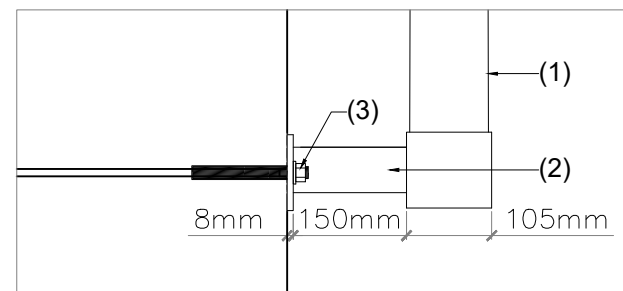
FLAGPOLE FIXING DETAILS 1:10
