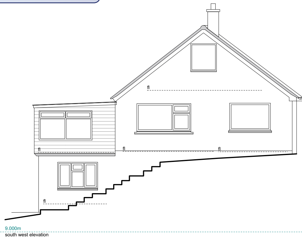
EXISTING SOUTH WEST ELEVATION SCALE: 1:100
