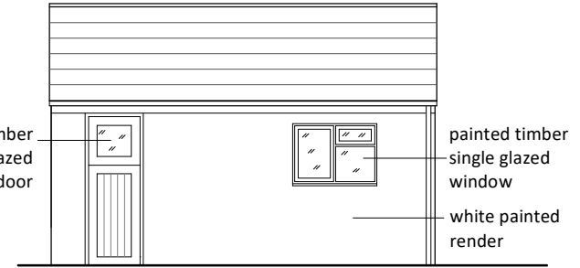
Elevation to side garden
