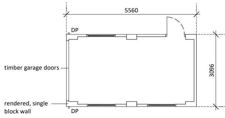
Existing Garage Plan
