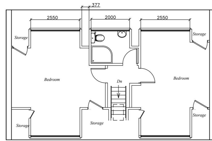
Roof Space
