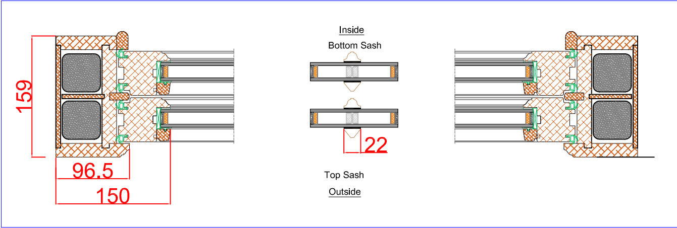
Timber Vertical Sliding Sash
