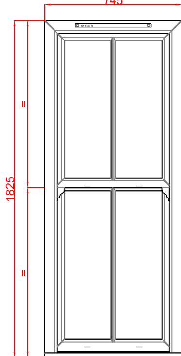
Frame Type 22
