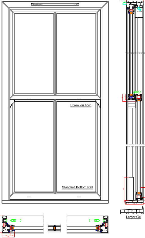
Standard window - with Horns
