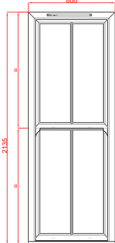
Frame Type 19
