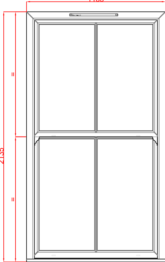
Frame Type 20
