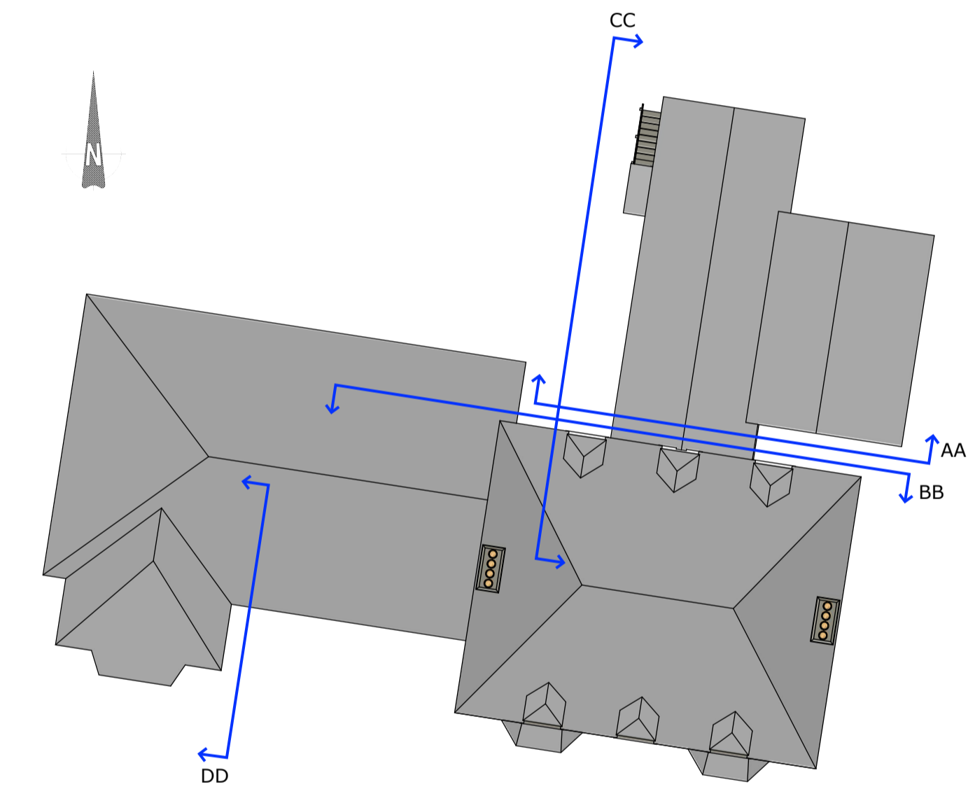
Roof Plan 1:200
