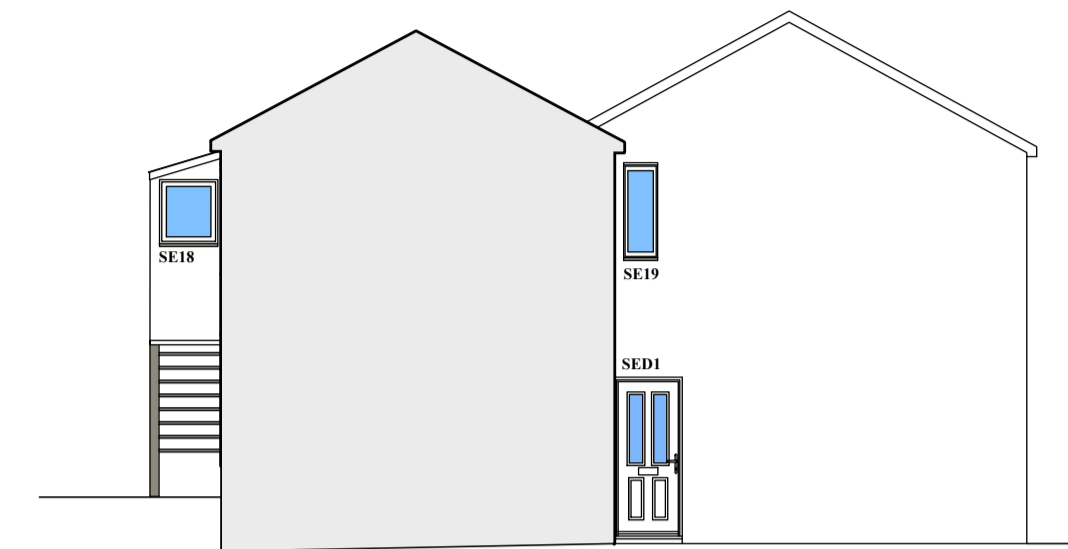
AA South Elevation 1:100
