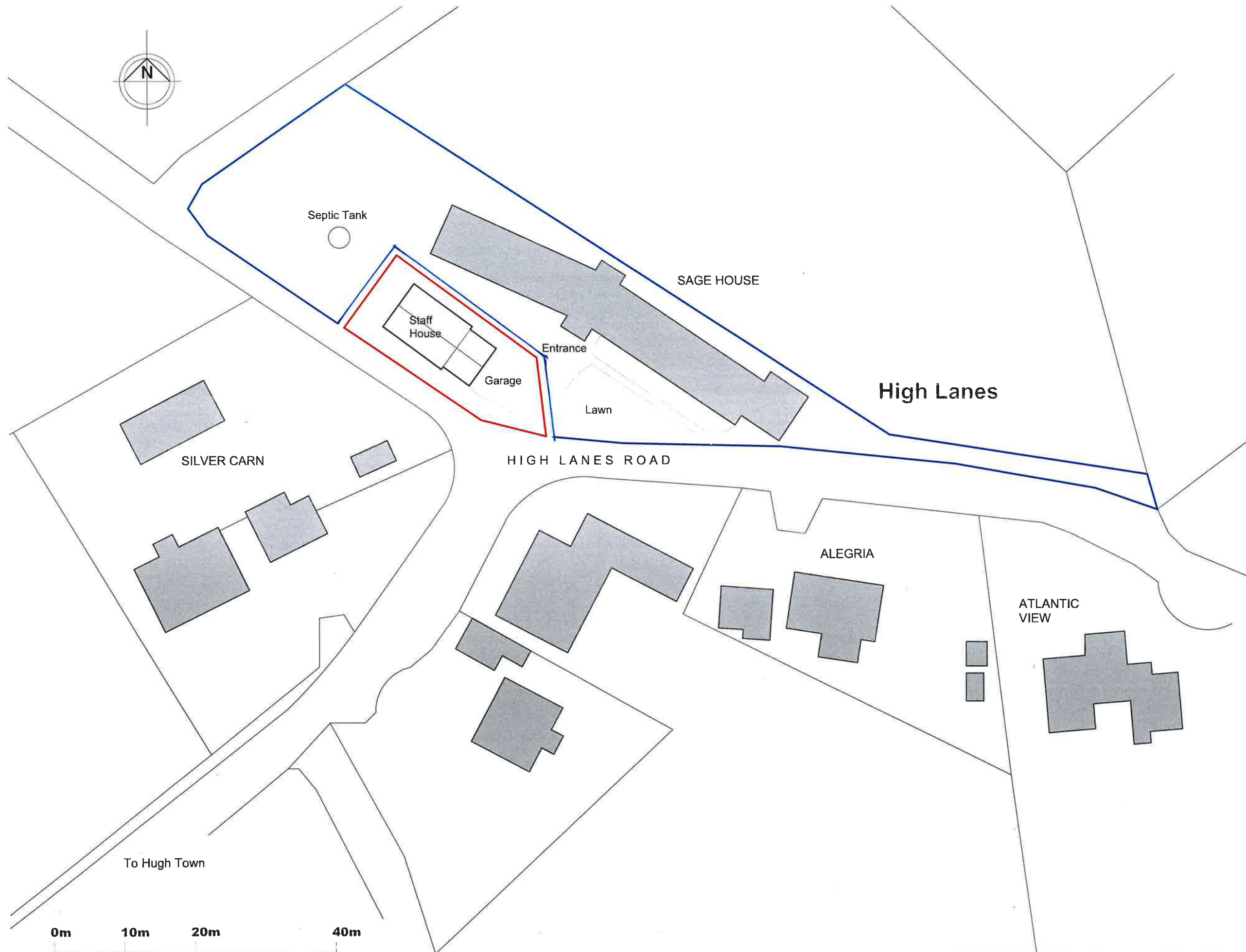
Site Plan
