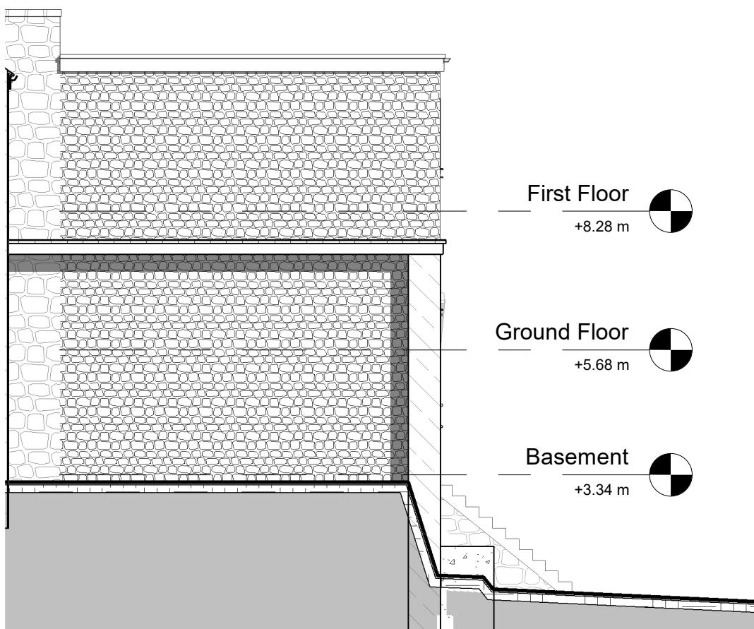
2 Existing South-East Elevation 1 : 100
