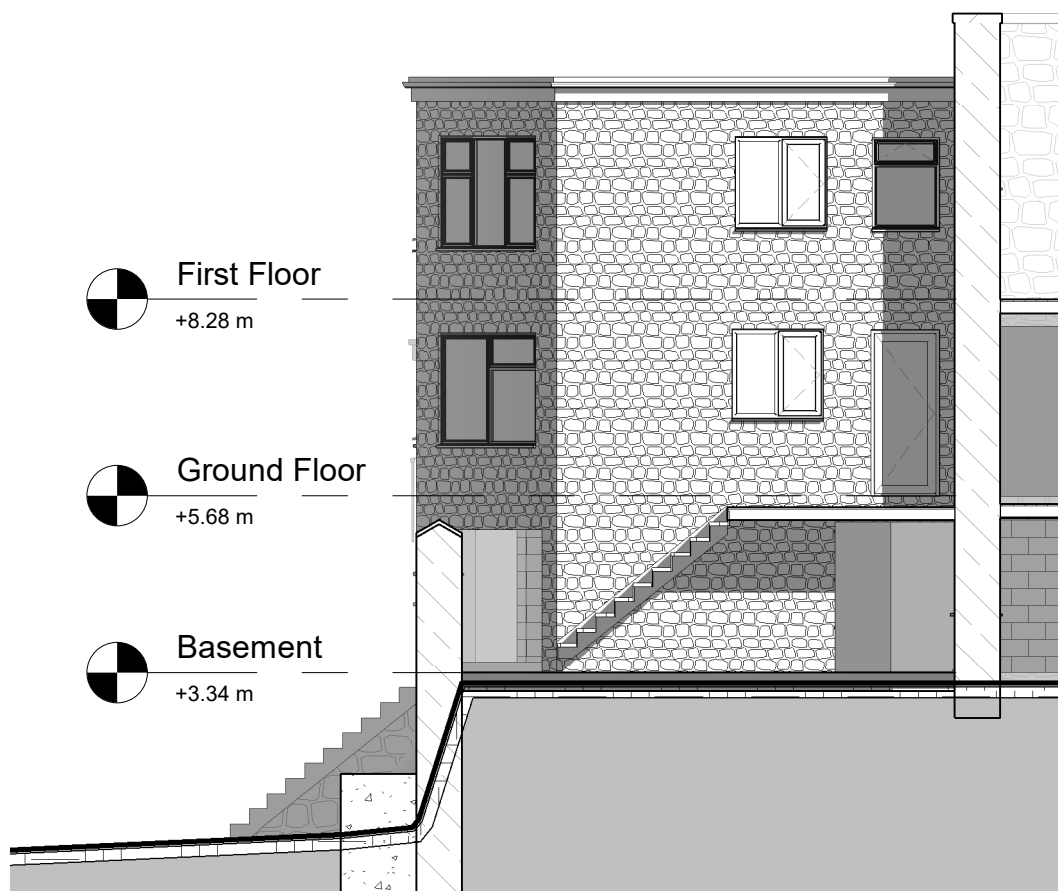
1 Existing North-West Elevation 1 : 100
